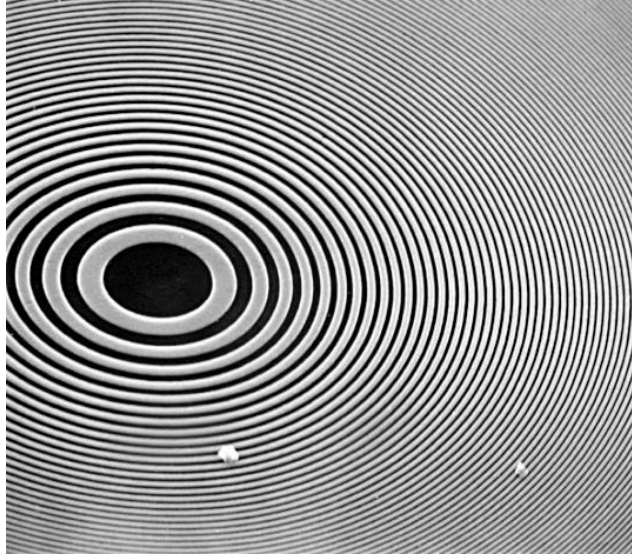
Figure 4 Scanning electron microscope image of the inner part of a Fresnel Zone Plate Lens. This lens has 318 nickel zones, a diameter of 45 \mu\text{m} , and the smallest (outermost) zone is 35 nm wide. Image obtained from http://www-cxro.lbl.gov/microscopy/zp.gif
