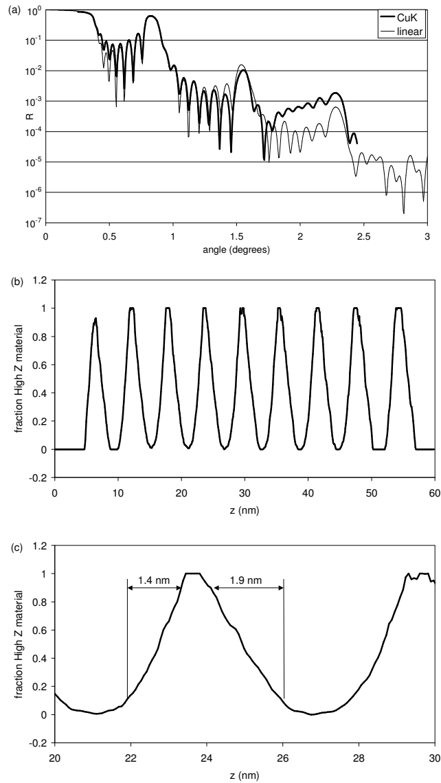
Figure 15 a Measured (thick line), and fitted (thin line) \theta/2\theta reflectivity curves at 0.154 nm ( \text{CuK}\alpha ).
