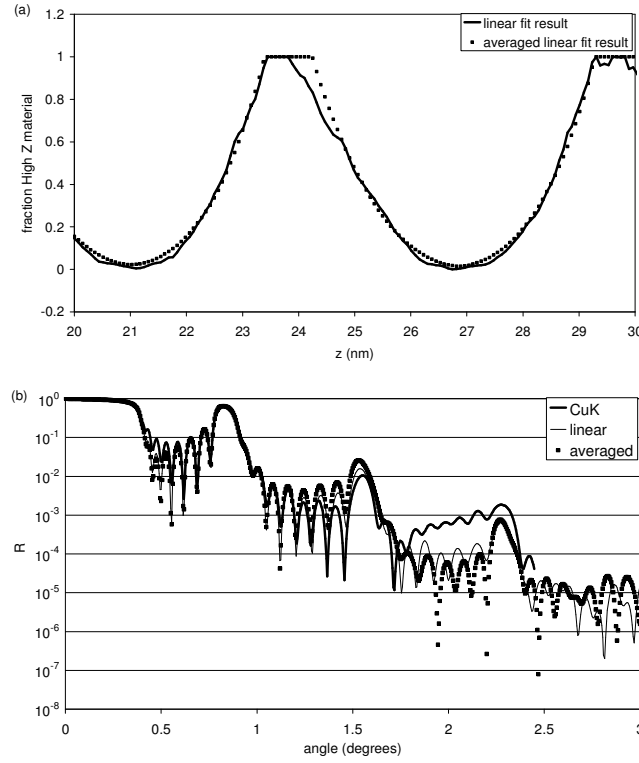
Figure 19a Comparison of the result of the analysis (a) of the W/Si multilayer using the original TEM input profile (solid line) and the 2 nm averaged TEM input profile (dotted line).
