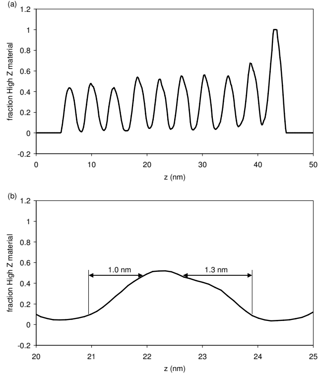
Figure 16a Calibrated tungsten concentration profile of the full multilayer stack. Clearly visible is the difference between the first (deepest) W layer, which is not treated with ions, and the subsequently deposited layers, which are treated with 1000 eV \text{Kr}^+ ions.
