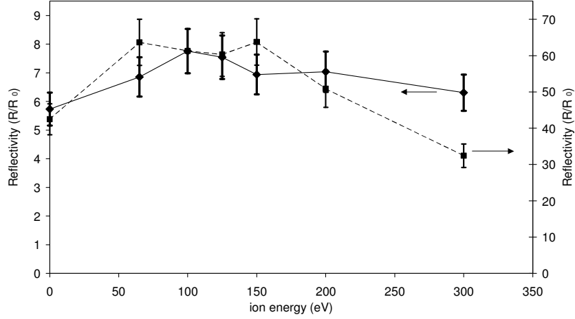
Figure 23 Peak in-situ reflectivity as a function of ion energy applied during the deposition of W in Si/W/Si tri-layers (♦ and solid line) and 10-period stacks (■ and dashed line). The values at 300 eV are obtained using ion treatment after deposition of the W layer.
